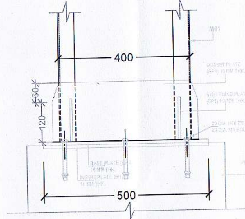
VIEW B1-B1 THROUGH THE BASE PLATE (BP1)
