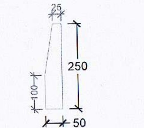
CUTTING DETAIL OF STIFFENING PLATE (SP2)
