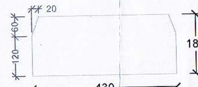
CUTTING DETAIL OF GUSSET PLATE (GP1)
