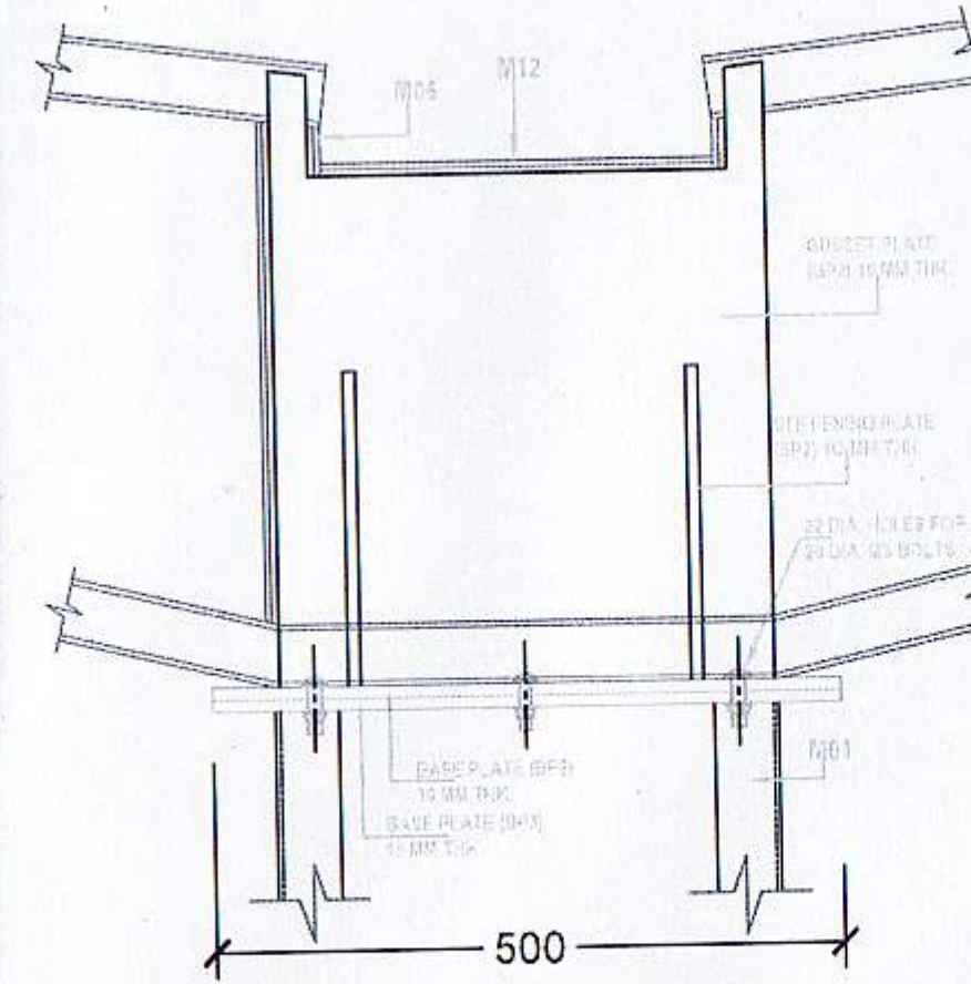
VIEW D1-D1 THROUGH THE BASE PLATE (BP2)
