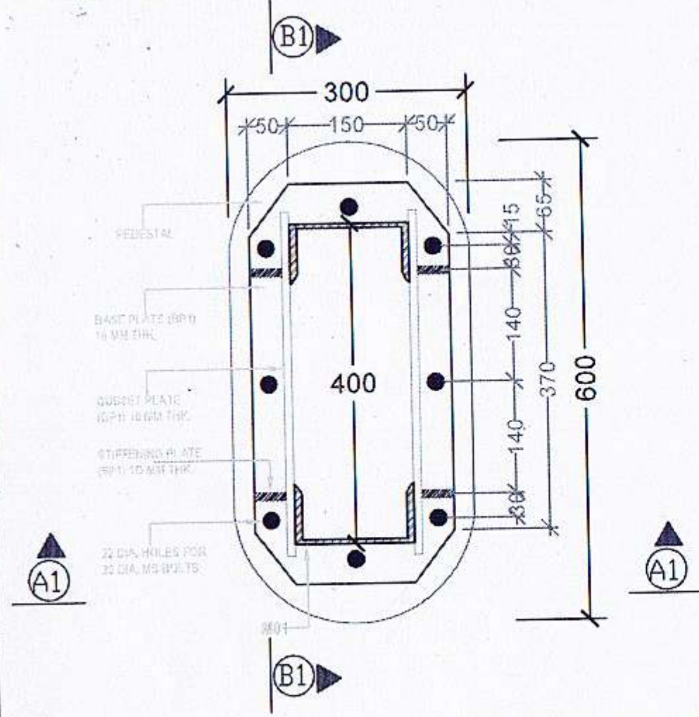
LAYOUT OF BASE PLATE (BP1) AT THE PEDESTAL
