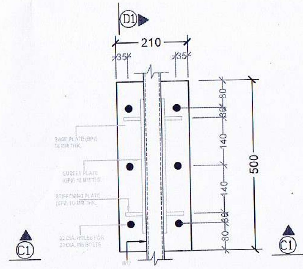
LAYOUT OF BASE PLATE (BP2) AT THE COLUMN
