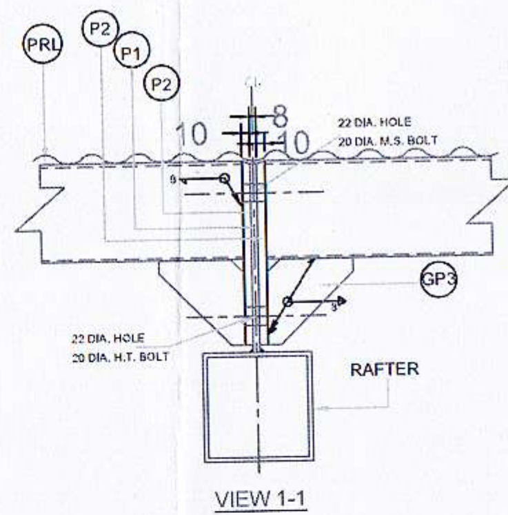
VIEW 1-1
