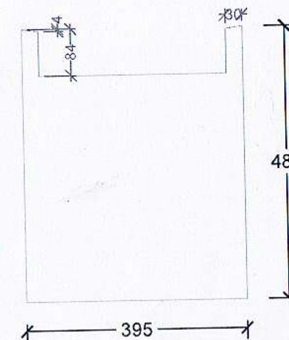
CUTTING DETAIL OF GUSSET PLATE (GP2)
