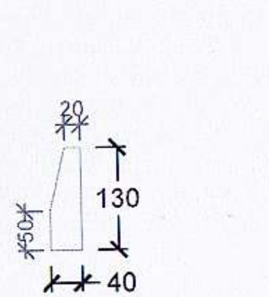
CUTTING DETAIL OF STIFFENING PLATE (SP1)
