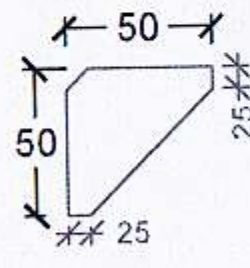
CUTTING DETAIL OF GUSSET PLATE (GP3)
