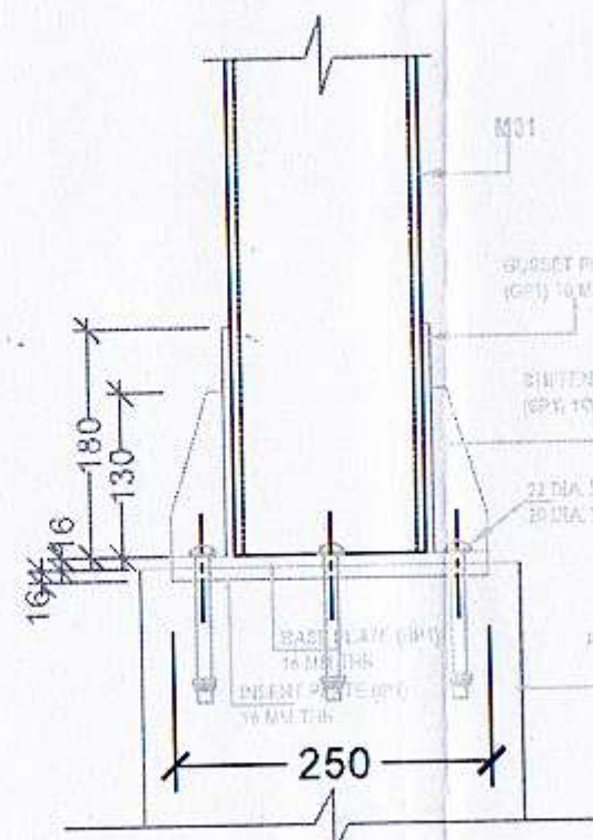
VIEW A1-A1 THROUGH THE BASE PLATE (BP1)
