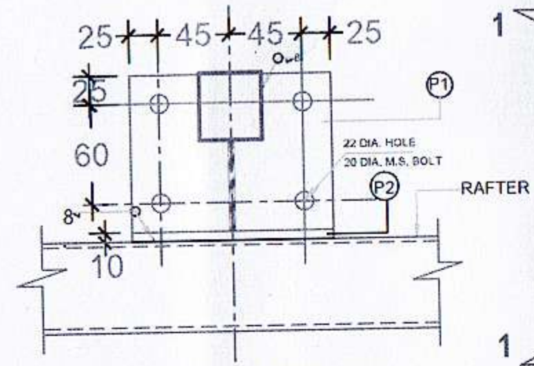
CONNECTION BETWEEN PURLIN & TRUSS T1
