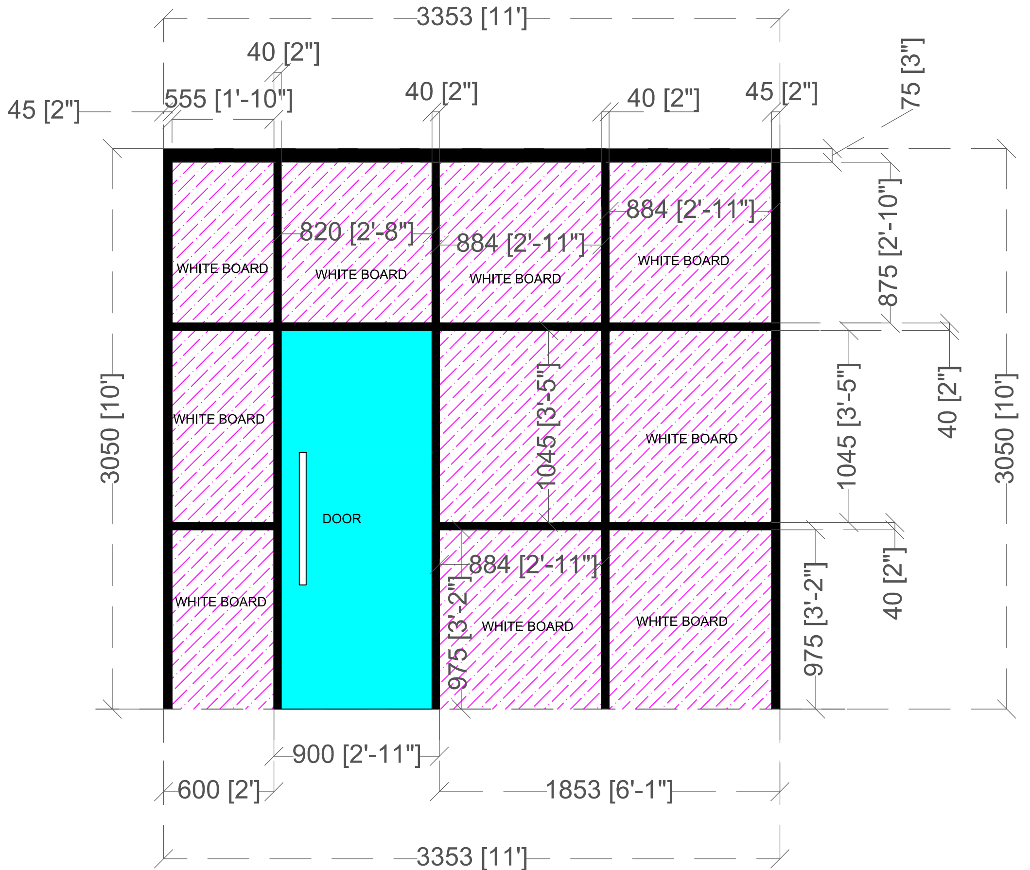
ALLUMINIUM PARTITION FRAME FOR UPS ROOM
